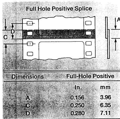
Figure 1 Dimensions and location of transverse cemented splices in 35 mm film.
