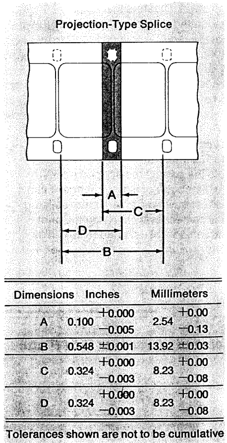
Figure 2 Dimensions and location of transverse cemented splices in 16 mm film.
