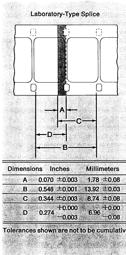
Figure 2 Dimensions and location of transverse cemented splices in 16 mm film.
