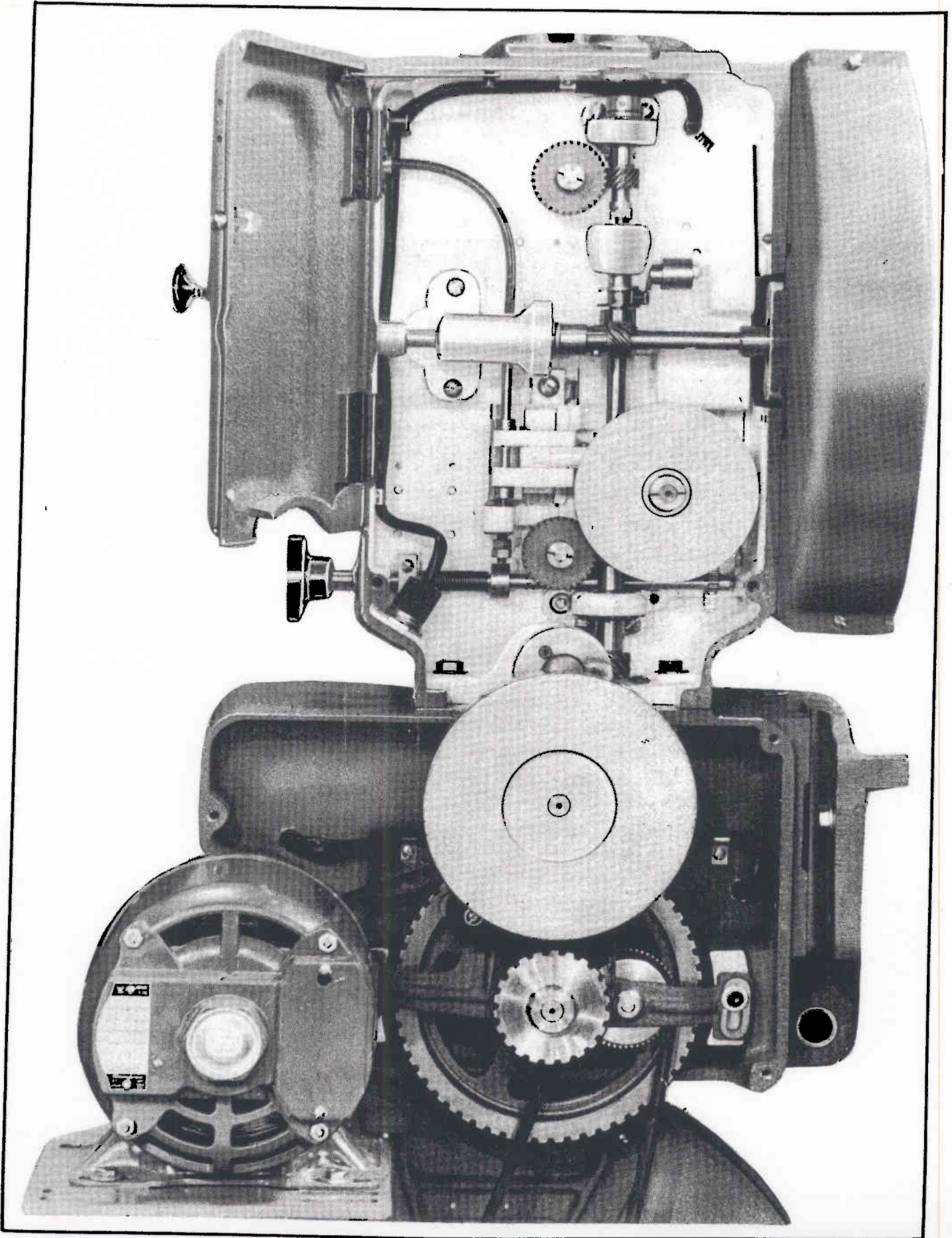
CENTURY PROJECTOR MECHANISM AND CENTURY SOUND REPRODUCER SINGLE SHUTTER-DRIVE SIDE
