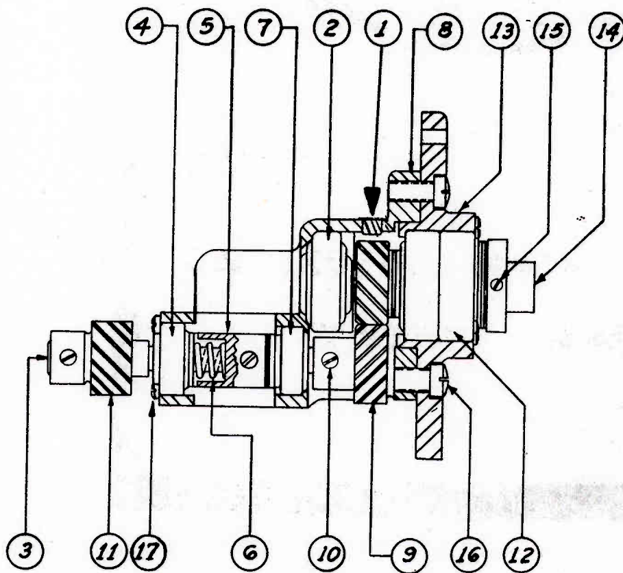
DOUBLE SHUTTER INTERMEDIATE GEAR BRACKET
