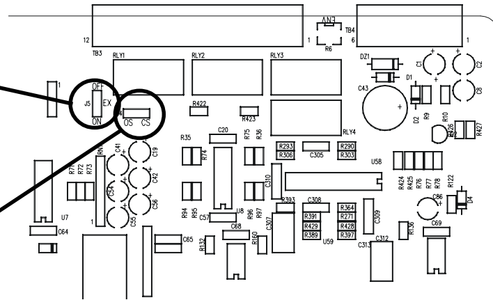
EX and Overhead Surround Jumper Settings Right Rear Corner of Main Board
