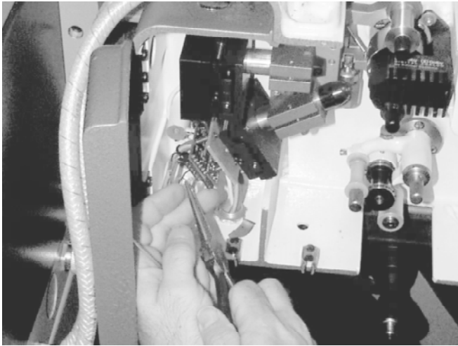
Connecting the MOD 7 to a Reverse Scan soundhead.
