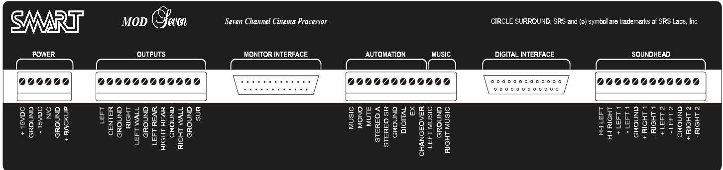
MOD 7 rear panel
