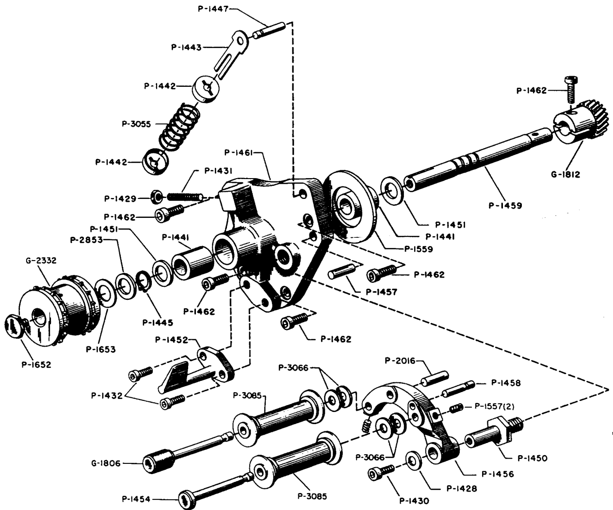
G-1809 LOWER FEED SPROCKET PARTS
