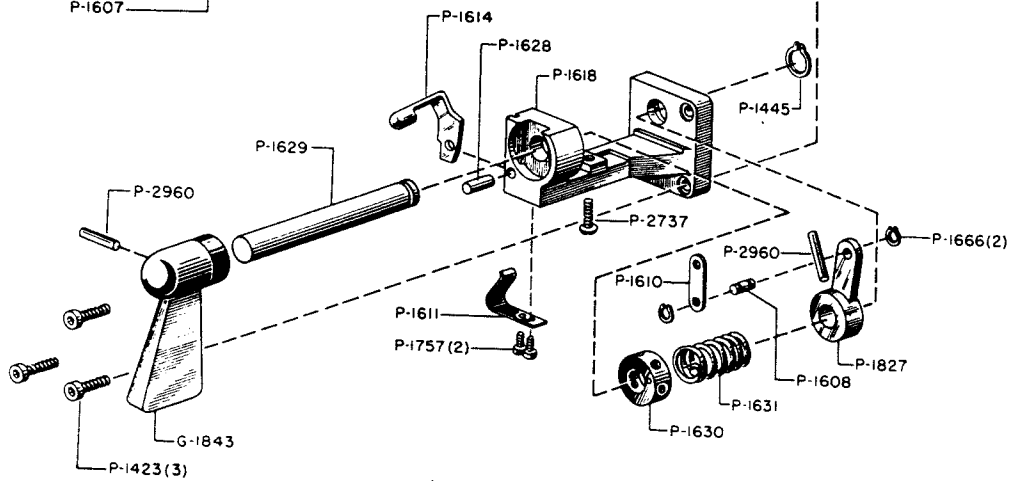
G-1905 FILM TRAP AND DOOR MOUNTING AND OPERATING ASSEMBLY
