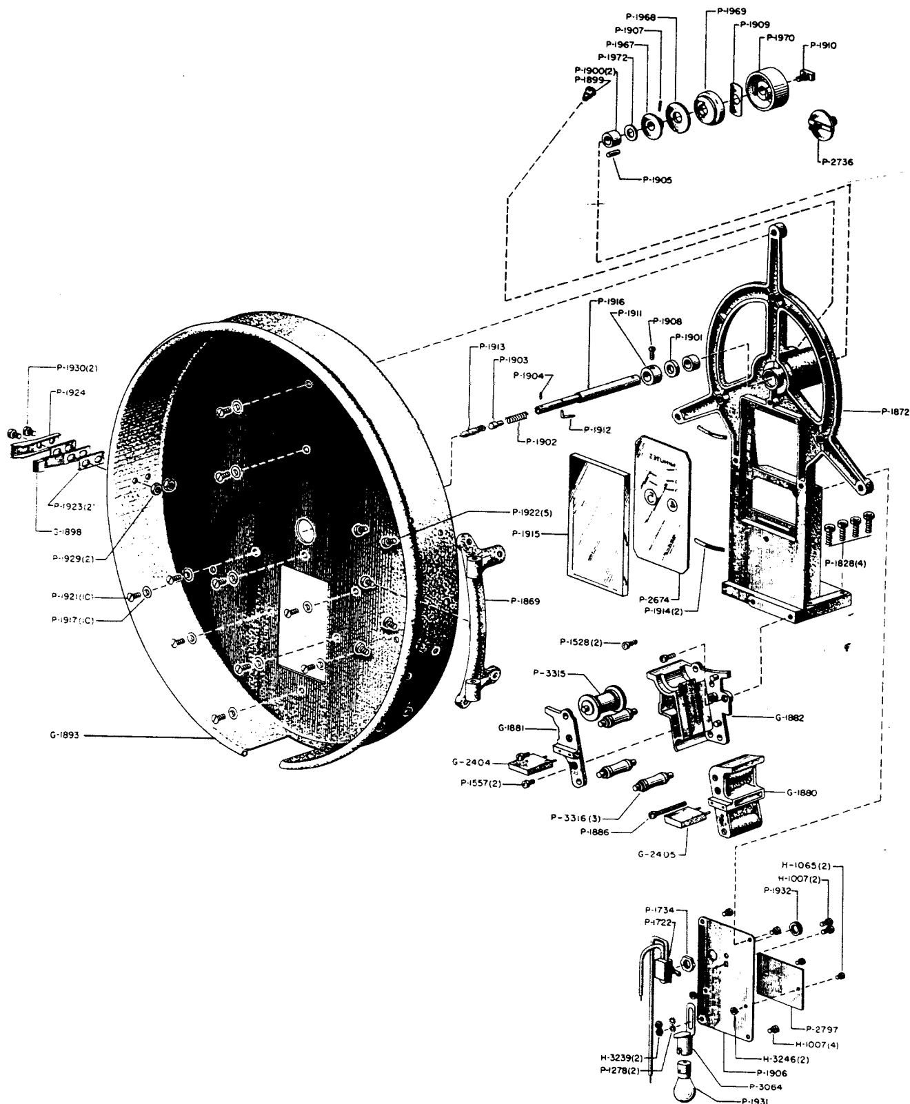
X-L UPPER MAGAZINE AND ROLLER HOLDER ASSEMBLY
