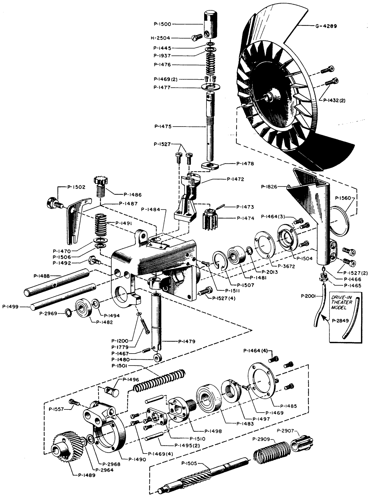
G-1815 SHUTTER AND FRAMING ASSEMBLY
