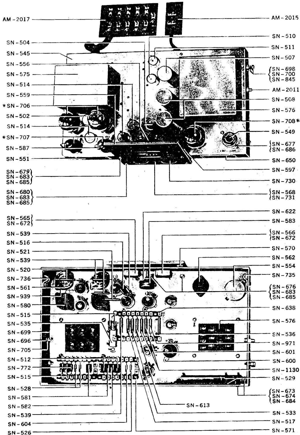
AM-1001 POWER AMPLIFIER
