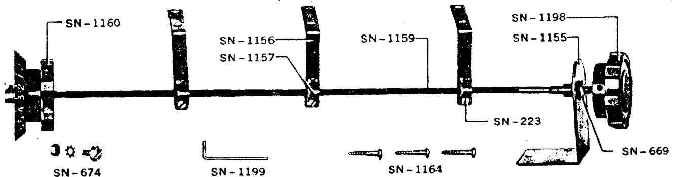
AM-2082 EXTENSION VOLUME CONTROL
