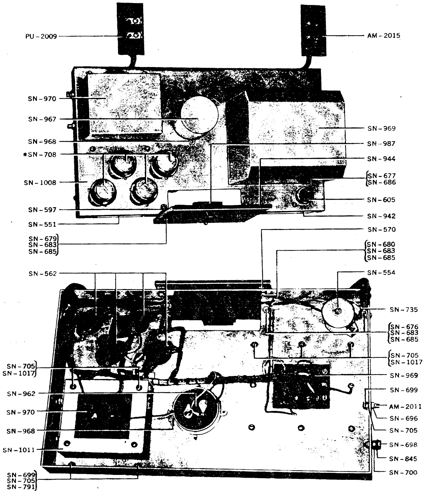
PU-1003 POWER UNIT
