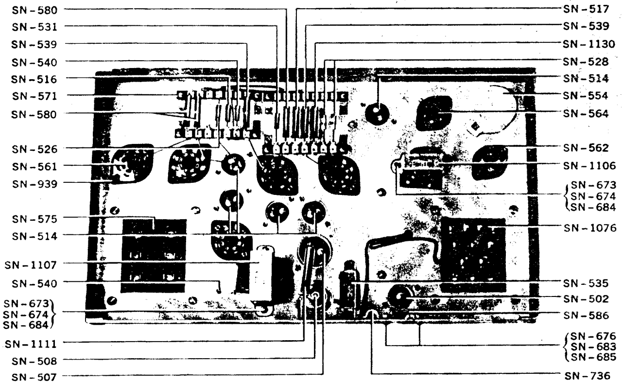
AM-1011 POWER AMPLIFIER
