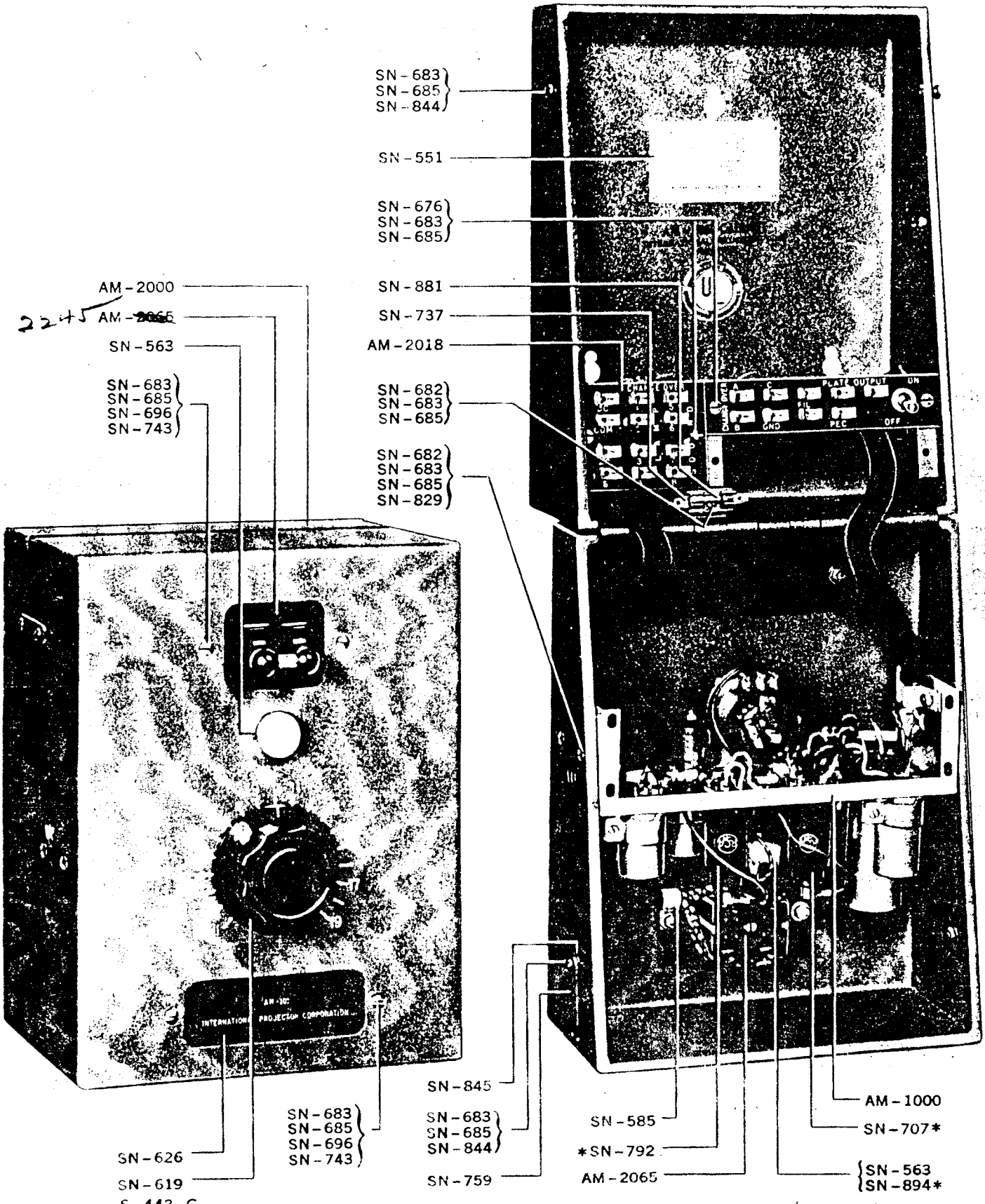
AM-101 VOLUME CONTROL AMPLIFIER
