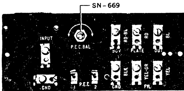
AM-2074 TERMINAL STRIP ASSEMBLY
