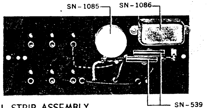
AM-2074 TERMINAL STRIP ASSEMBLY
