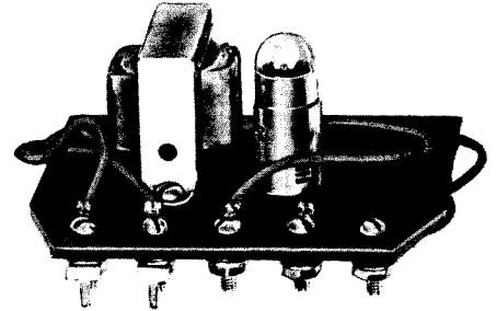
TERMINAL STRIP WITH DOWN LIGHT AND TAPER TABS TERMINALS
