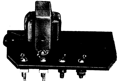
TERMINAL STRIP LESS DOWN LIGHT WITH TAPER TAB TERMINALS
